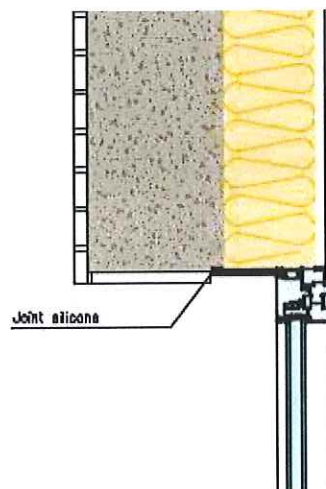
Figure 7 — Linteau
