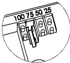
Daughterboard jumper
