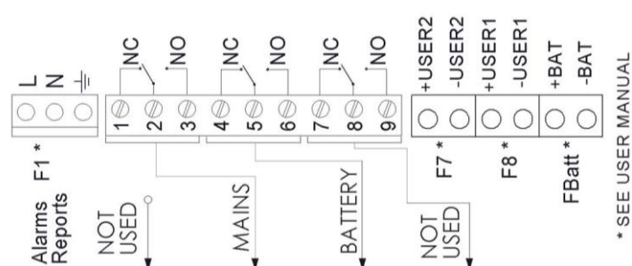
Alarm reports wiring
