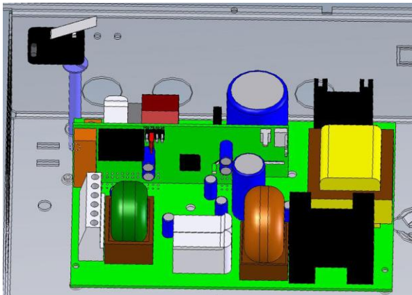
C24 Switch
