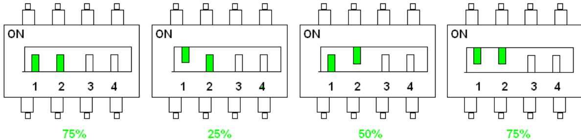
Figure 3: configuring battery current limitation using microswitches 1 & 2
