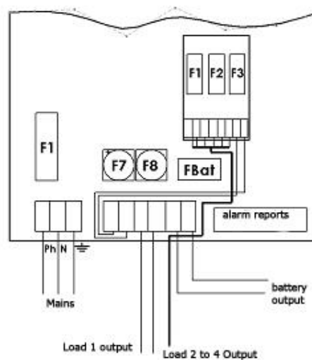
3-output board (fuse protected) – 75 W
