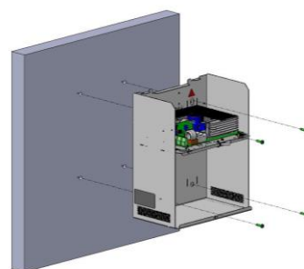
C7 – Dim : 243x194x97mm – IP30
