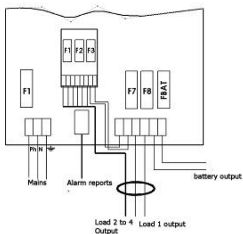
3-output board (fuse protected) 100-150 W
