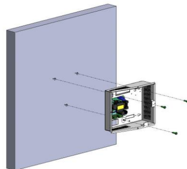
C7 – Dim : 243x194x97mm – IP30
