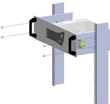
Rack 3U – Dim : 483x132x235mm (court) – IP30
