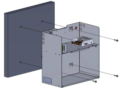
C85 – Dim : 408x408x224mm – IP31
