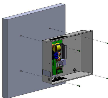
C48 – Afm: 425x345x120mm - IP30
