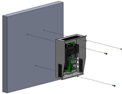
C23 – Abm: 248x322x126 mm – IP30
