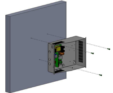
C24 - Abm : 322x248x126mm - IP 30
