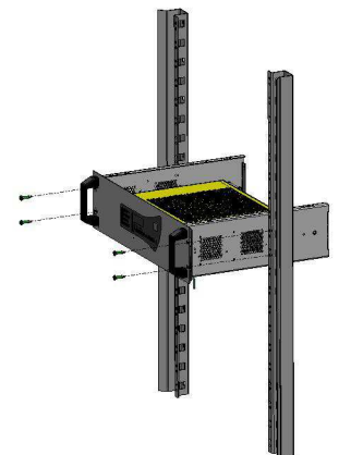
Rack 3U – Abm : 483x132x358mm – IP30
