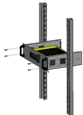
Rack 3U – Dim : 483x132x358mm – IP30
