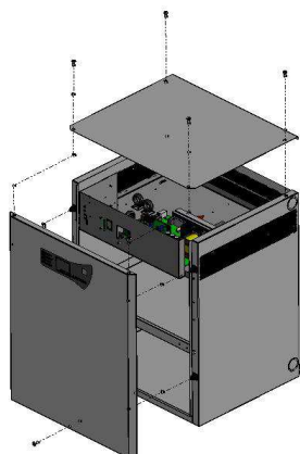
C180 – Afm: 505x610x430mm – IP31
