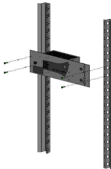
RackF3U – Dim : 482x133x110mm – IP30
