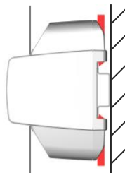
Figure 2: Clipped to DIN rail - side view
