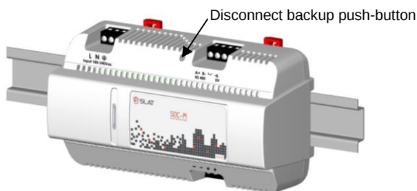
Figure 1: Clipped to DIN rail - front view
