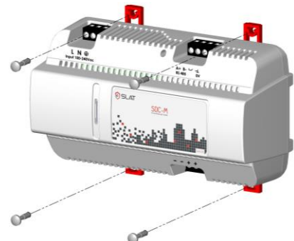
Figure 3: Fixed on mounting plate
