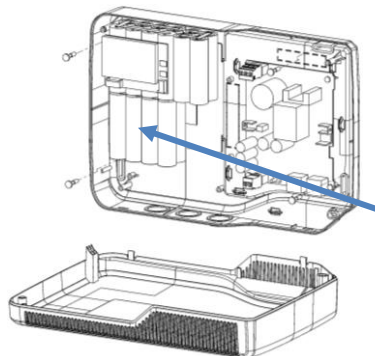
Fig. 1: Wall mounting
